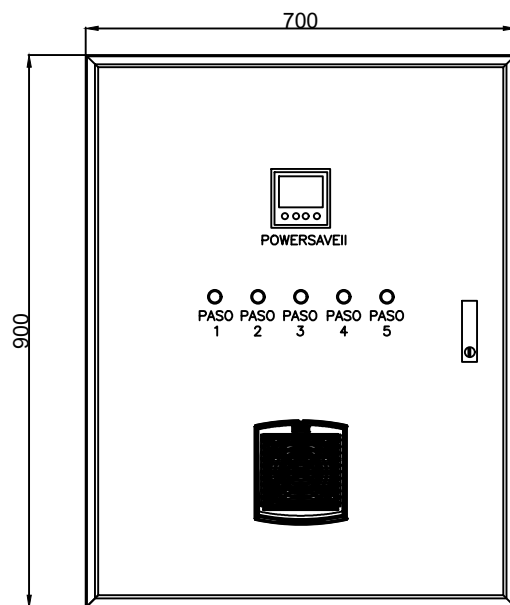
VISTA FRONTAL EXTERIOR
