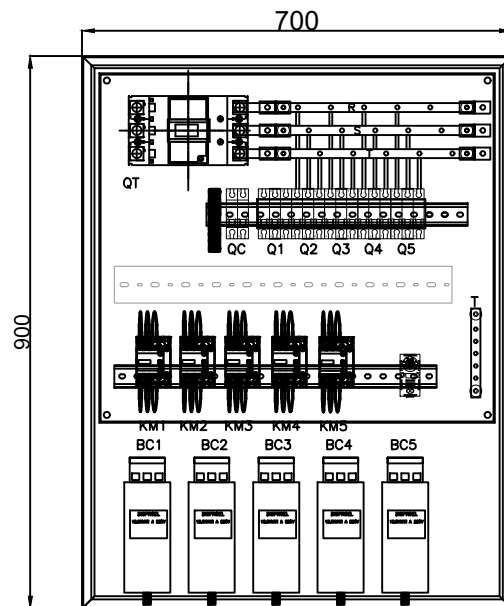
VISTA FRONTAL INTERIOR
